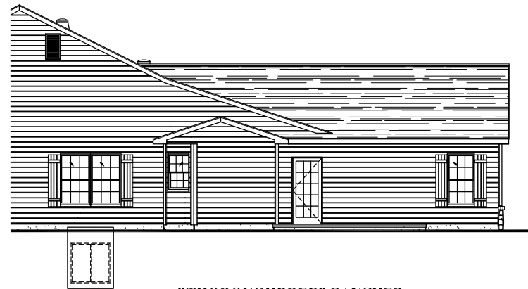
"THOROUGHbred" RANCHER SIDE ELEVATION
