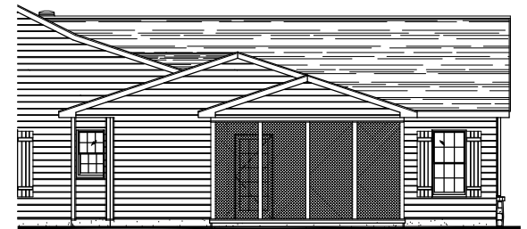
"THOROUGHbred" RANCHER W/ SCREENED-IN PATIO OPTION SIDE ELEVATION
